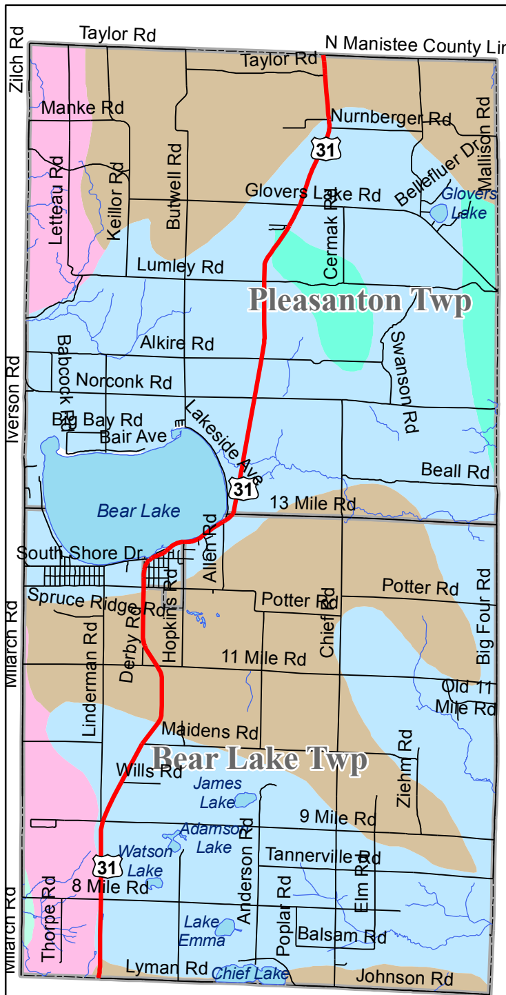
Bear Lake Community Map 8 Surface Geology
