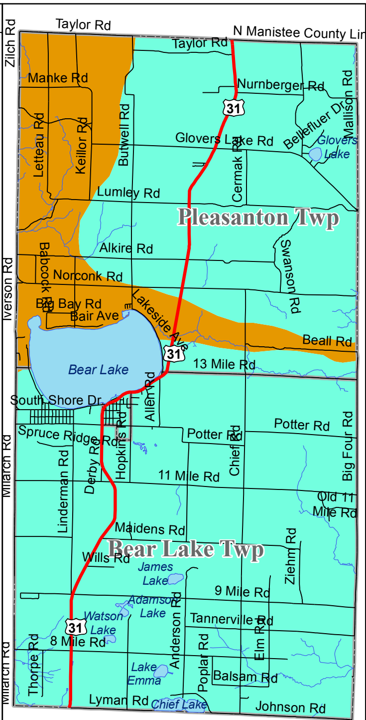
Bear Lake Community Map 8a Bedrock Geology
